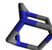
Methenamine
