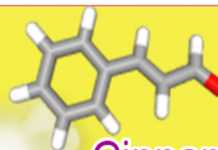
Cinnamaldehyde
