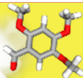
Asaraldehyde
