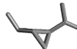
Thujone
